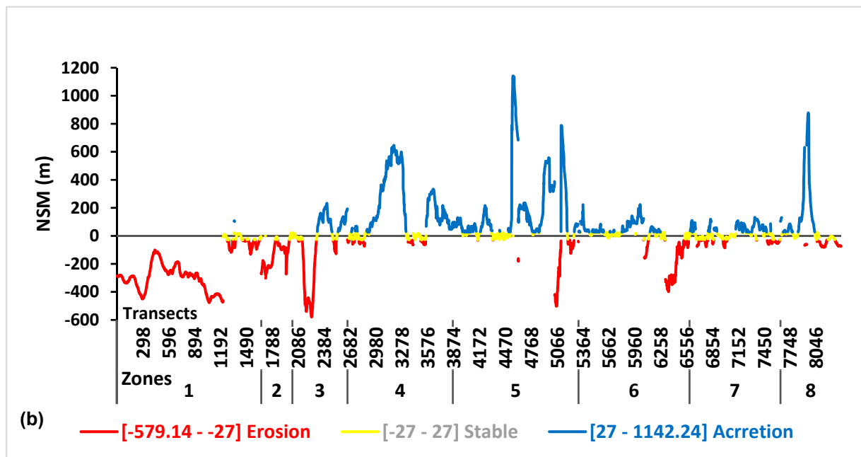
Figure 8. Shoreline evolution between 1948 and 2012 in the Wouri estuary, (erosion and accretion) computed by the EPR (a), NSM (b) methods.
